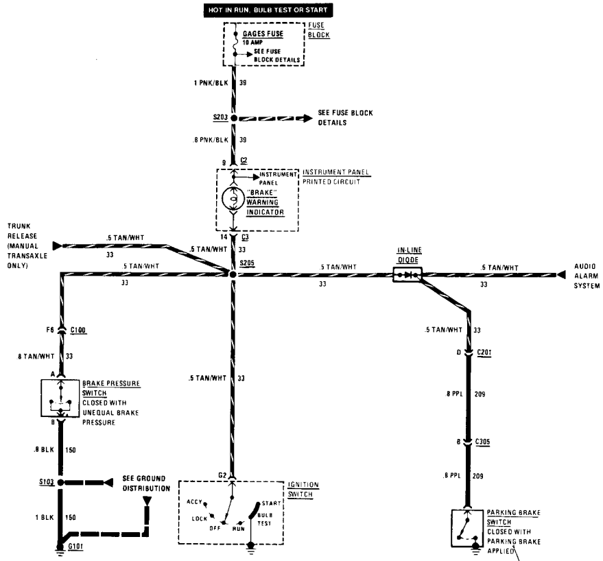
Brake warning system
