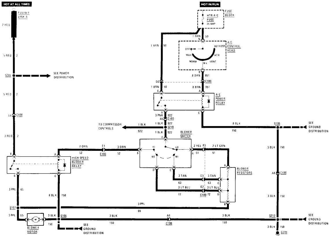
Air conditioning system - blower controls
