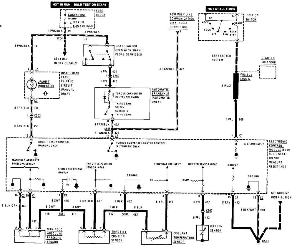
Electronic fuel injection (four-cylinder engine) — electronic data sensors, Torque Converter Clutch (TCC) and upshift indicator
