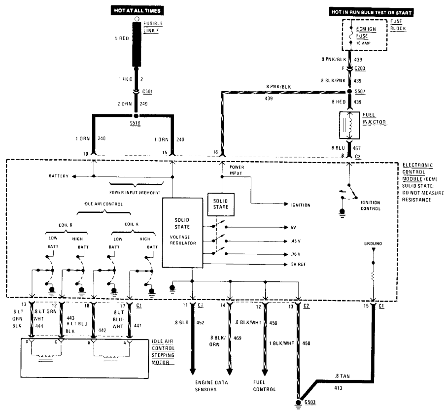
Electronic fuel injection (four-cylinder engine)
