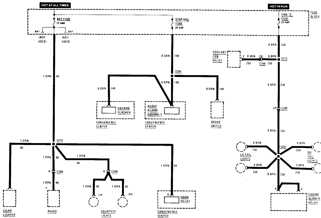
Fuse box details
