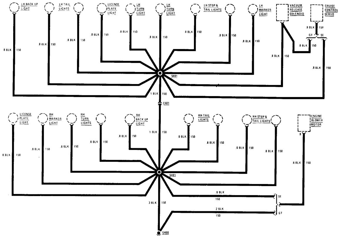
Ground distribution — rear lights
