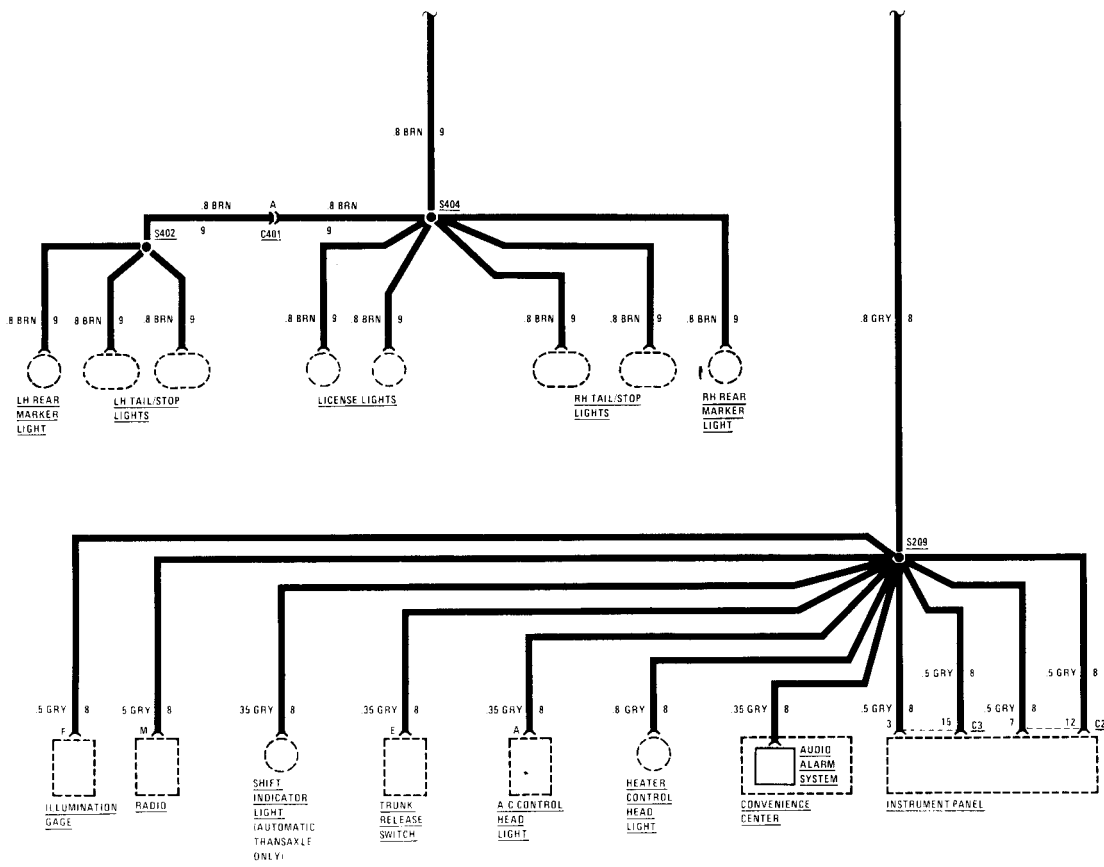
Light switch details
